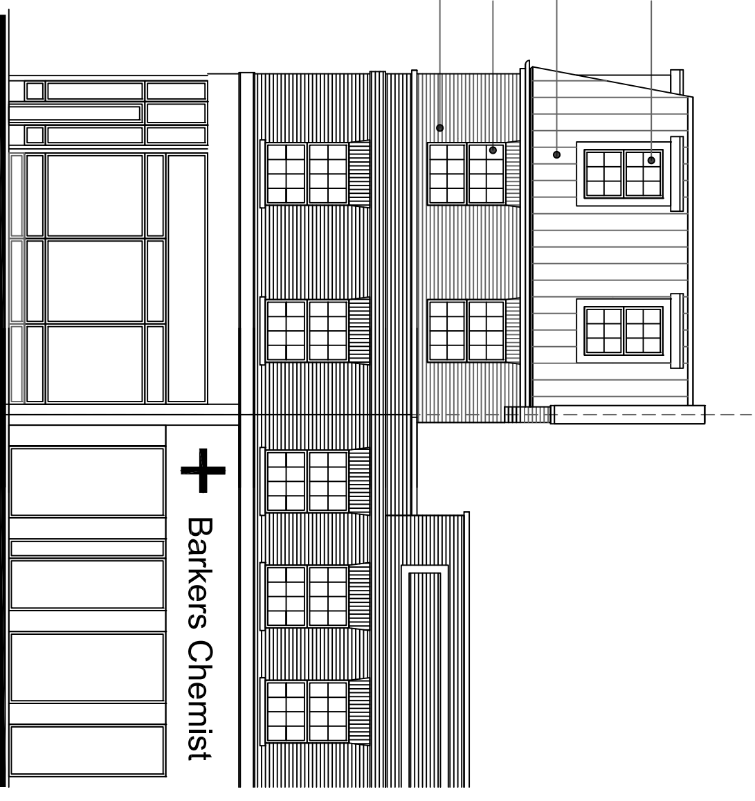
Front Elevation (south) Coombe Lane Elevation
