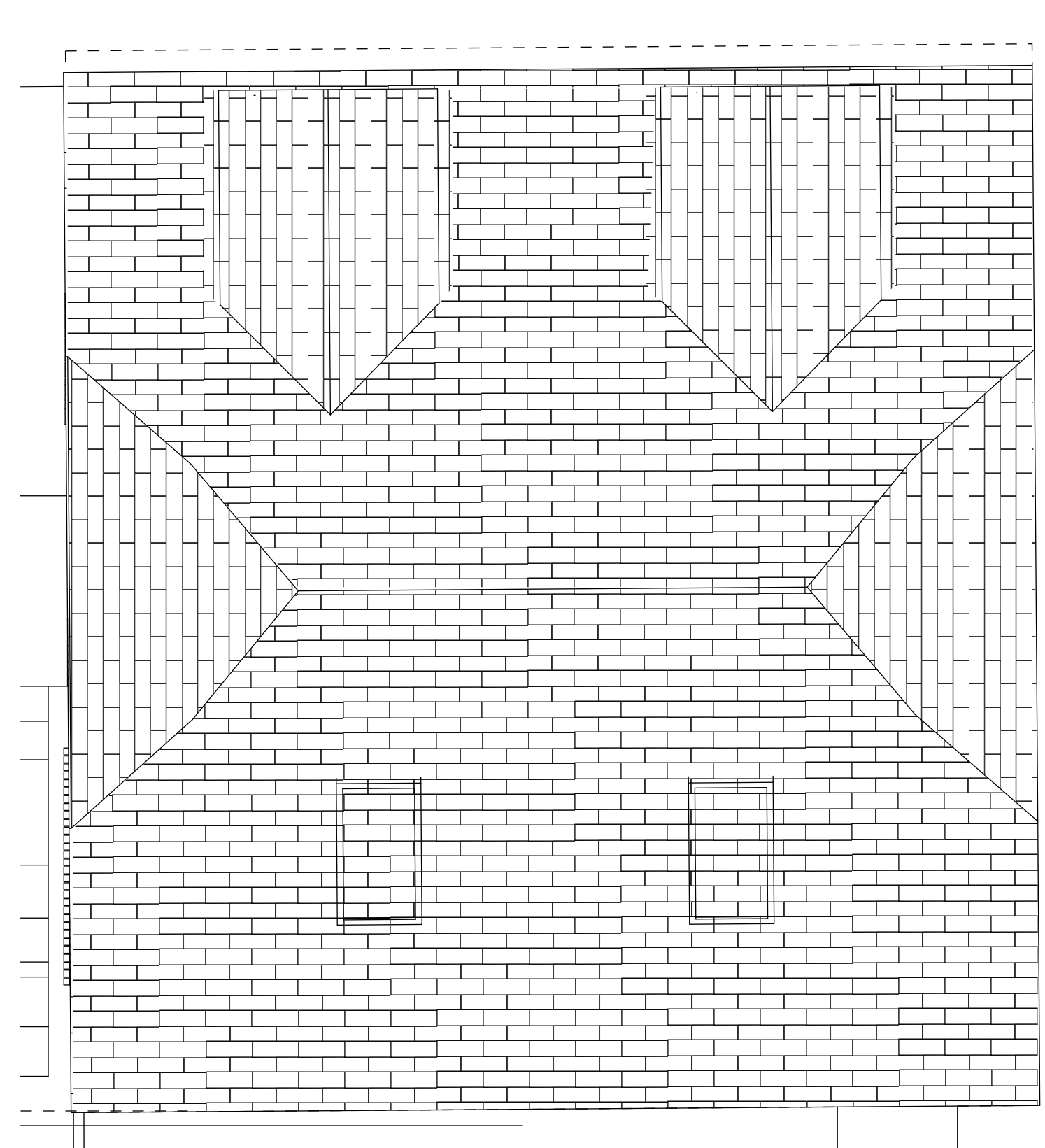
ROOF PLAN 1:50 @ A1/ 1:100@A3
