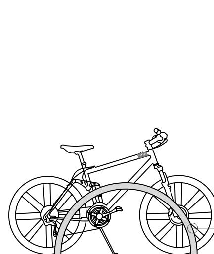
CYCLE RACK SIDE ELEVATION
