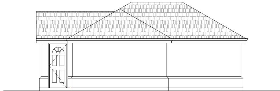
PROPOSED SOUTH-WEST ELEVATION
