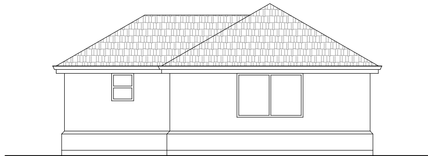
PROPOSED SOUTH-EAST ELEVATION
